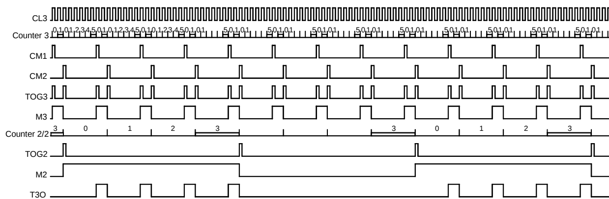
Figure 87. Burst Modulation 1
