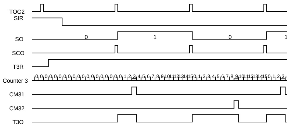
Figure 58. Pulse-width Modulation
