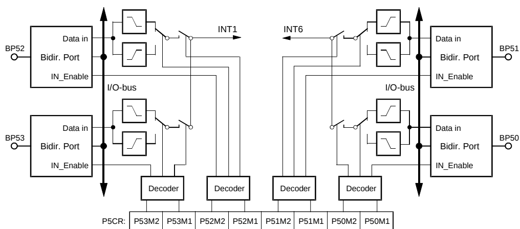
Figure 31. Port 5 External Interrupts
