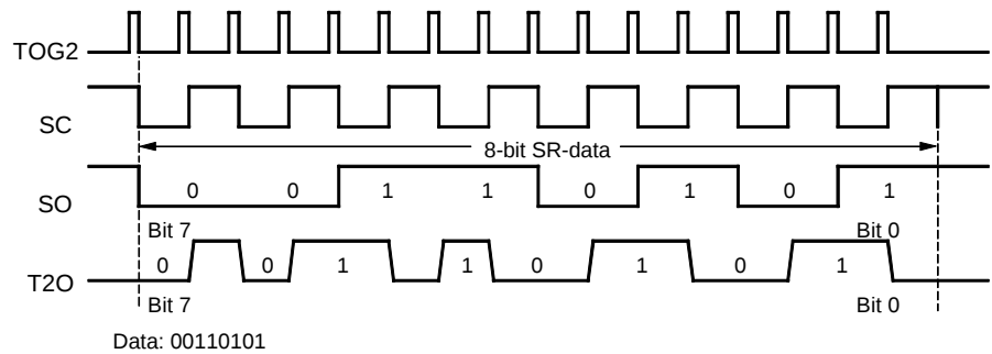
Figure 76. Manchester Modulation 1
