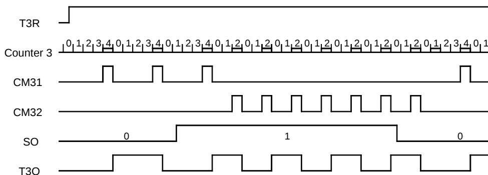
Figure 57. FSK Modulation
