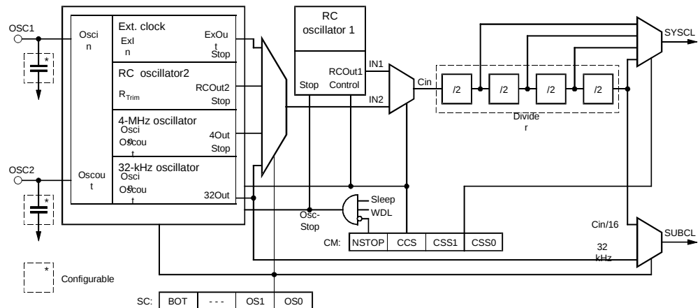
Figure 20. Clock Module
