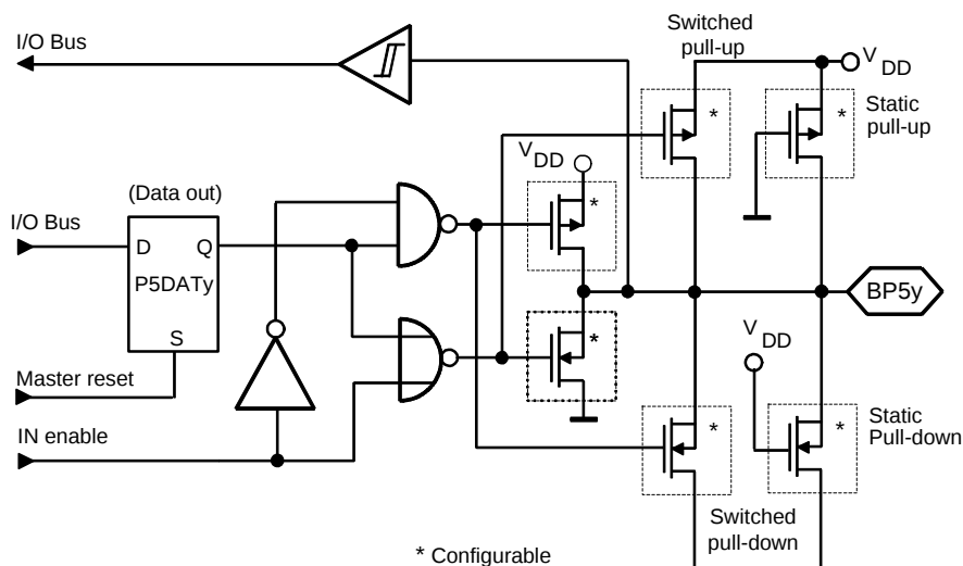
Figure 30. Bi-directional Port 5
