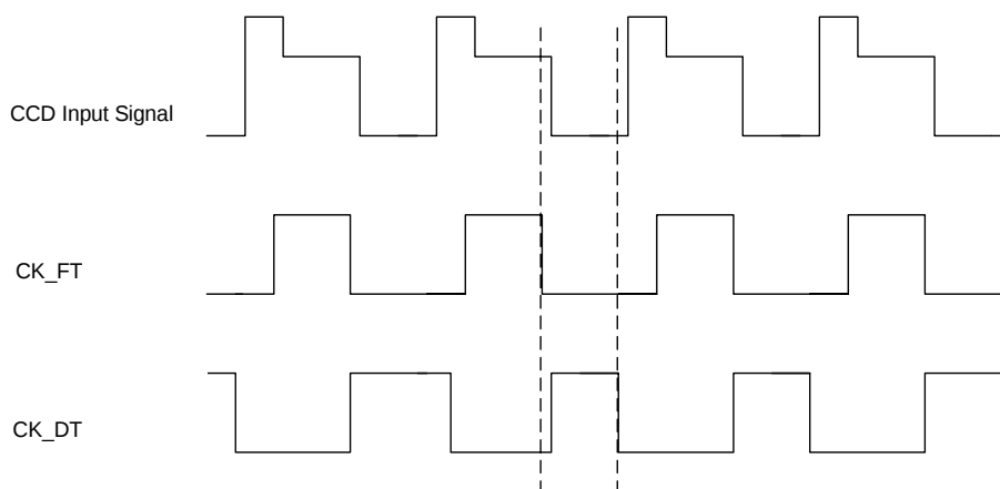
Figure 3. Clock Timing
