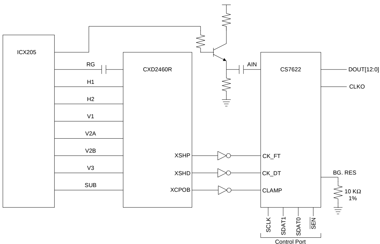
Figure 7. Connection Diagram
