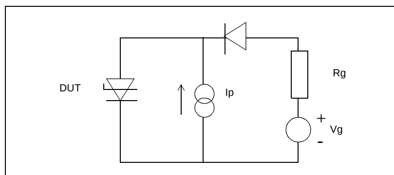
Figure 13 - Holding Current Circuit
