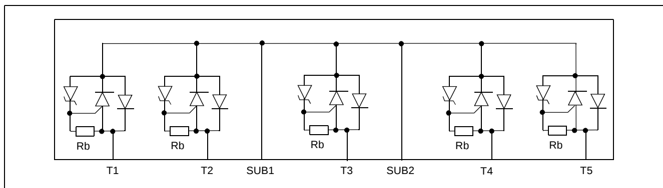
Figure 4 - ZL0008/ZL0009 Block Diagram
