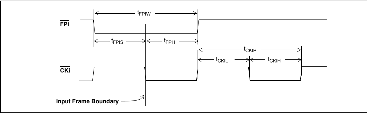
Figure 25 - Frame Pulse Input and Clock Input Timing Diagram
