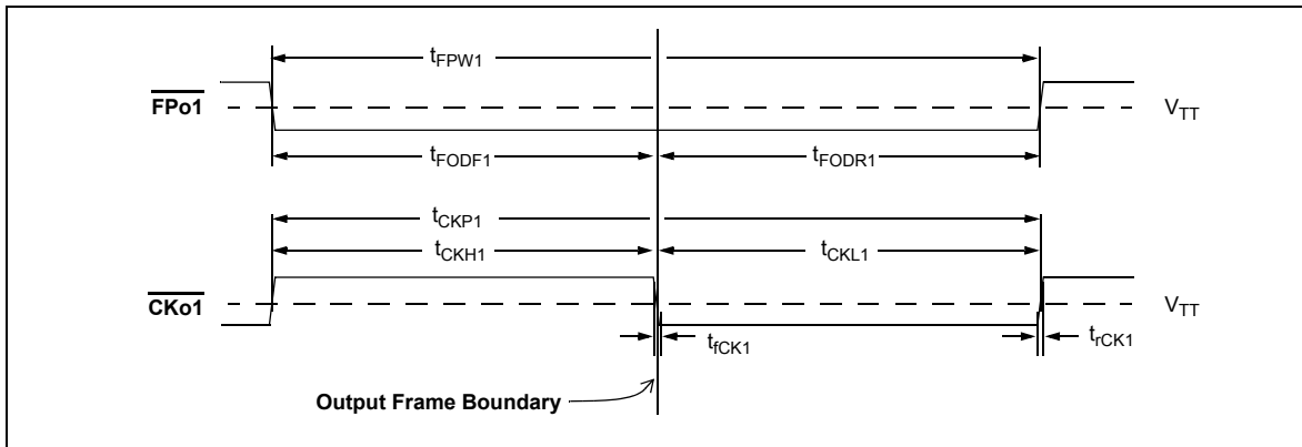
Figure 30 - \overline{\text{FPo1}} and \overline{\text{CKo1}} Timing Diagram
