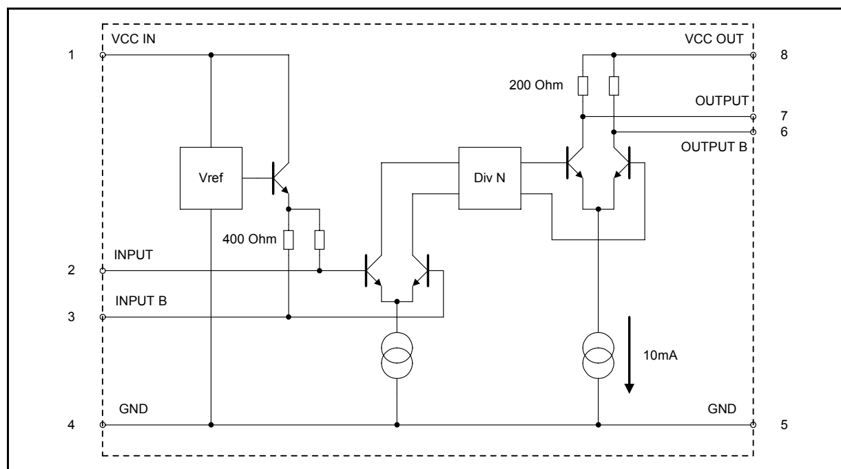
Figure 1 - Block Diagram
