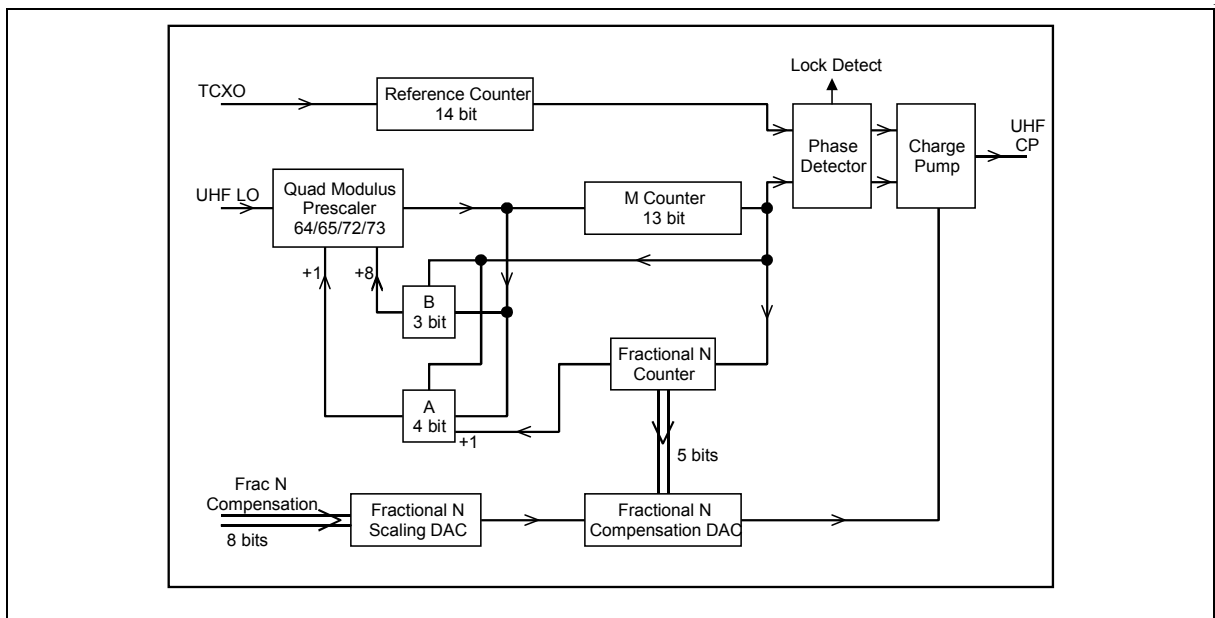
Figure 8 - UHF Synthesizer
