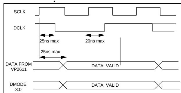
Figure 2. DBUS Timing
