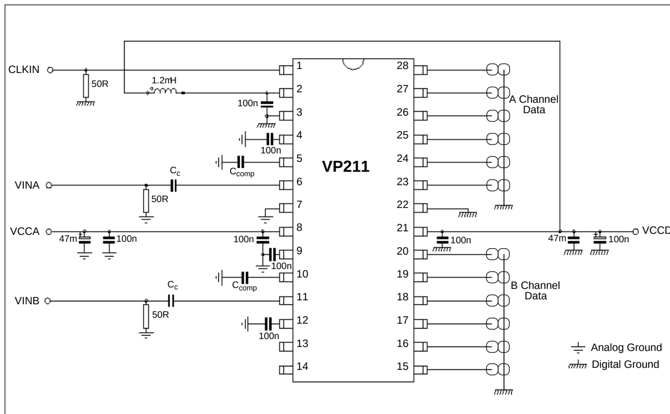
Fig.5 Applications diagram
