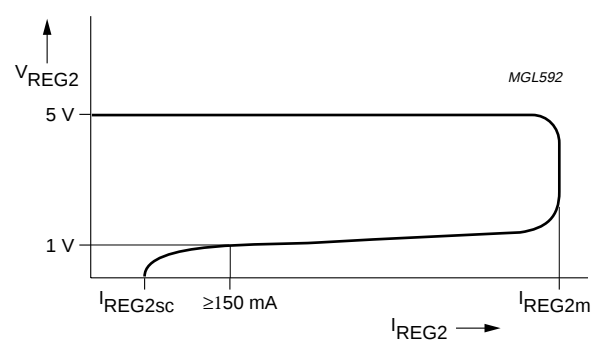
b. Regulator 2.
