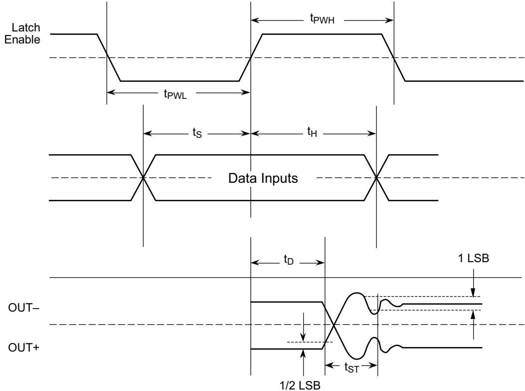
Figure 1 – Timing Diagram
