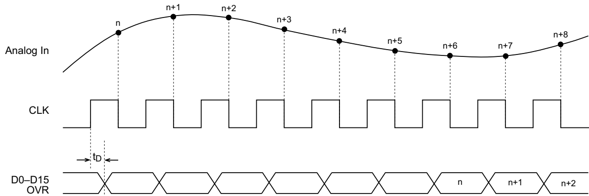
Figure 3 – Timing Diagram 1
