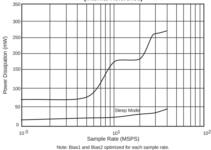
Power Dissipation vs Sample Rate (Internal Reference)
