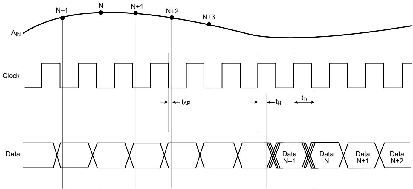
Figure 2 – Timing Diagram
