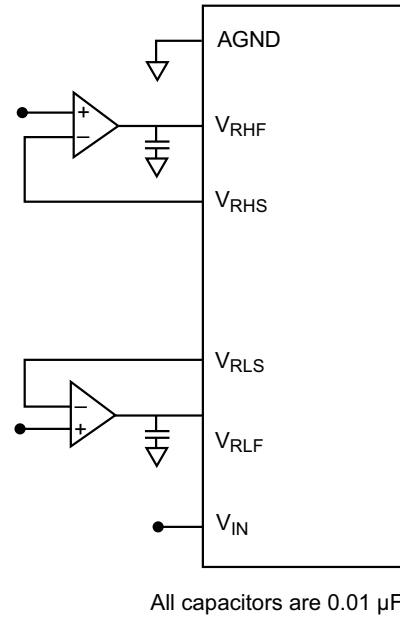
Figure 3 – Ladder Force/Sense Circuit
