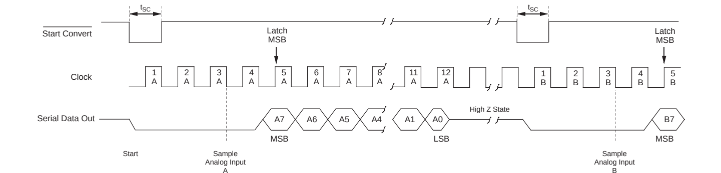
Figure 5 - Synchronous Mode Timing Diagram
