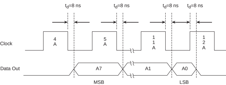
Figure 8 - Data Output Timing
