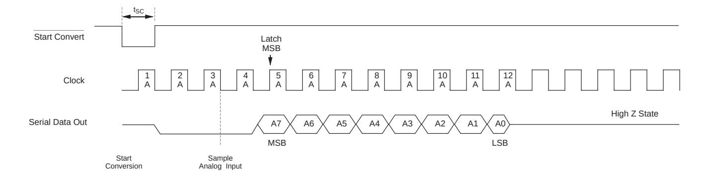
Figure 4 - Single Shot Mode Timing Diagram
