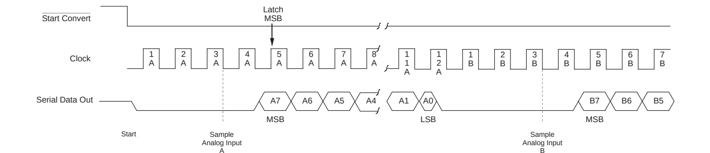
Figure 6 - Free Run Mode Timing Diagram
