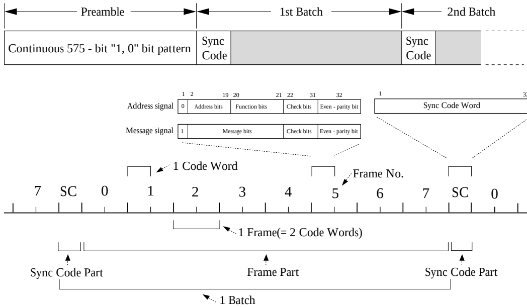
Figure 1. Receive signal format
