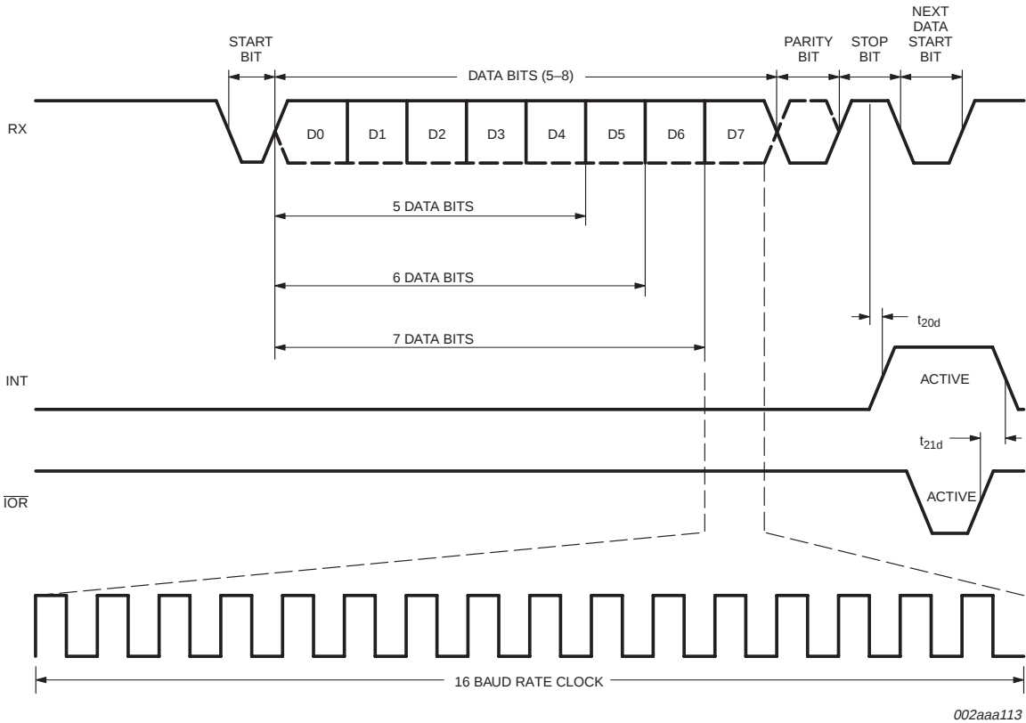
Fig 12. Receive timing.
