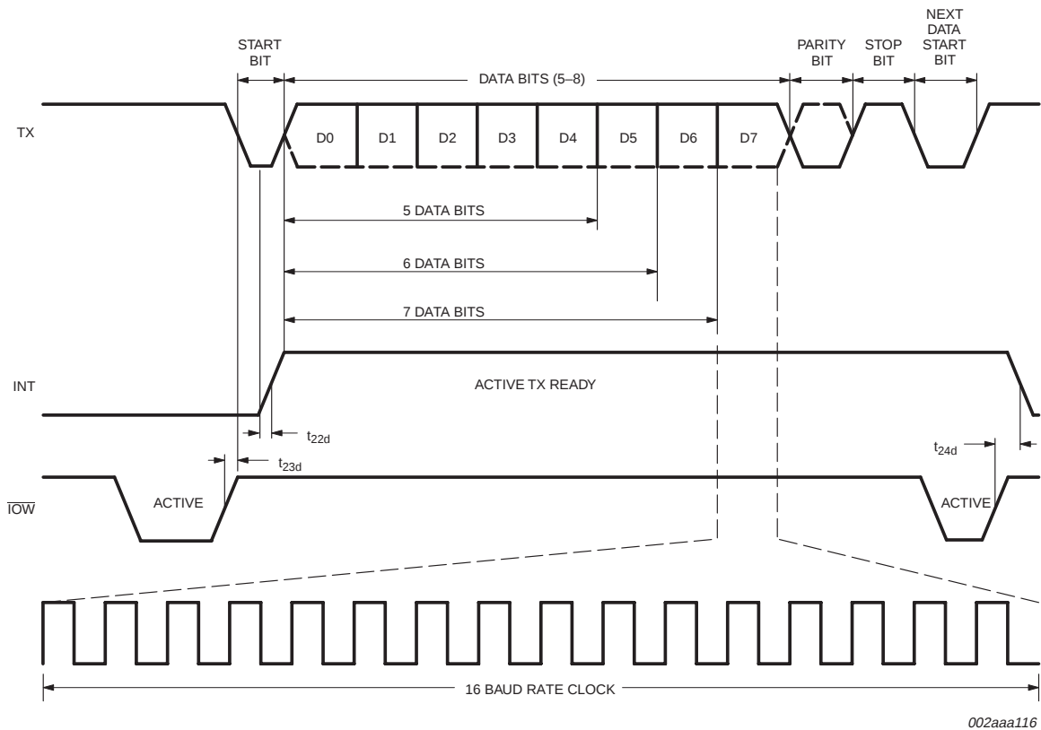
Fig 15. Transmit timing.
