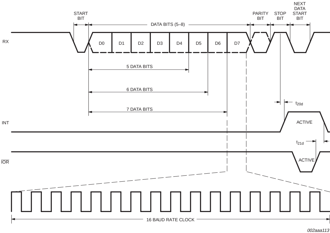
Fig 11. Receive timing.
