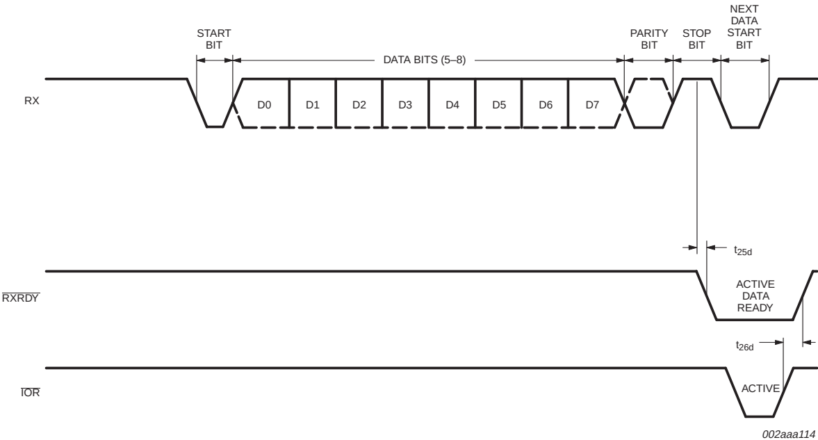
Fig 12. Receive ready timing in non-FIFO mode.
