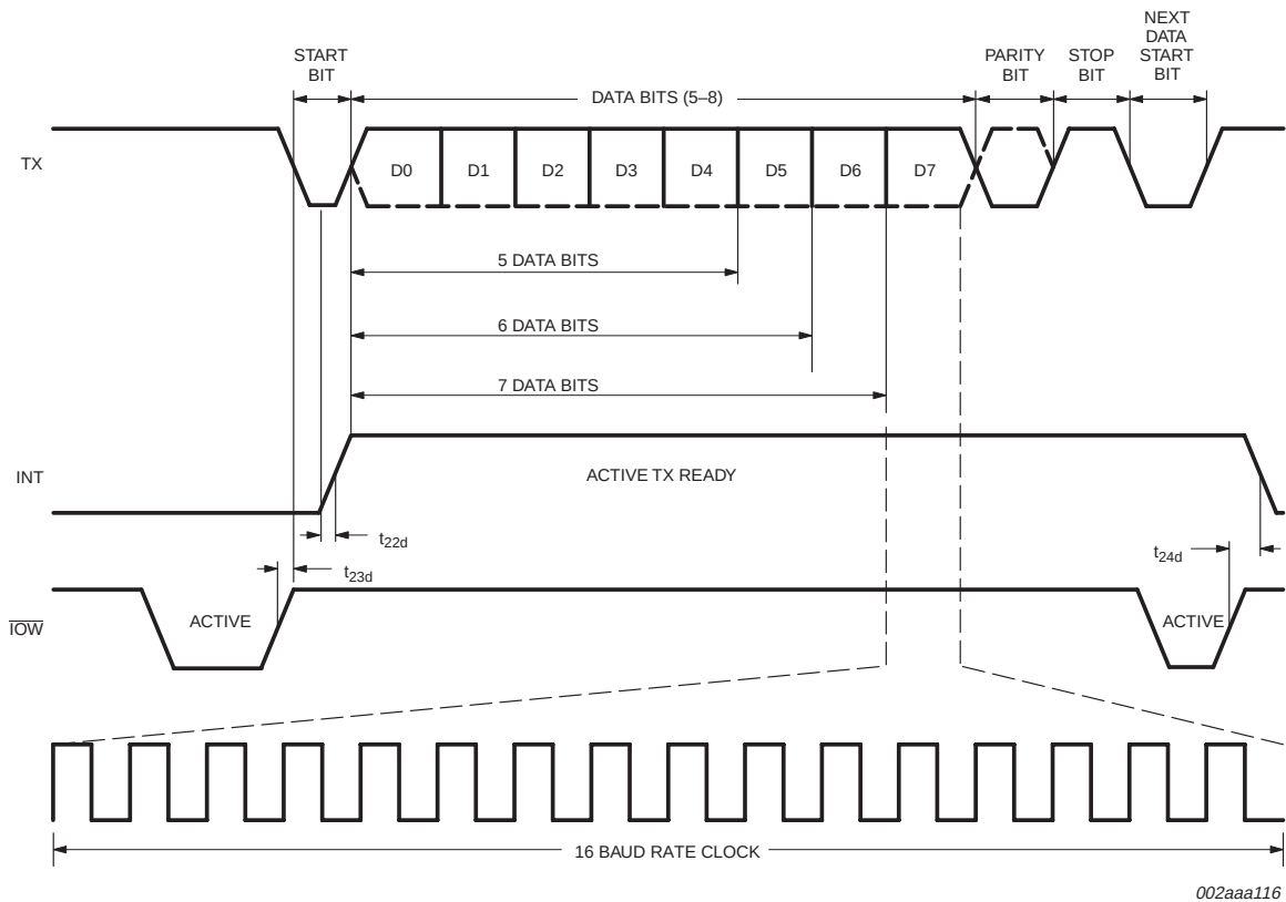
Fig 14. Transmit timing.
