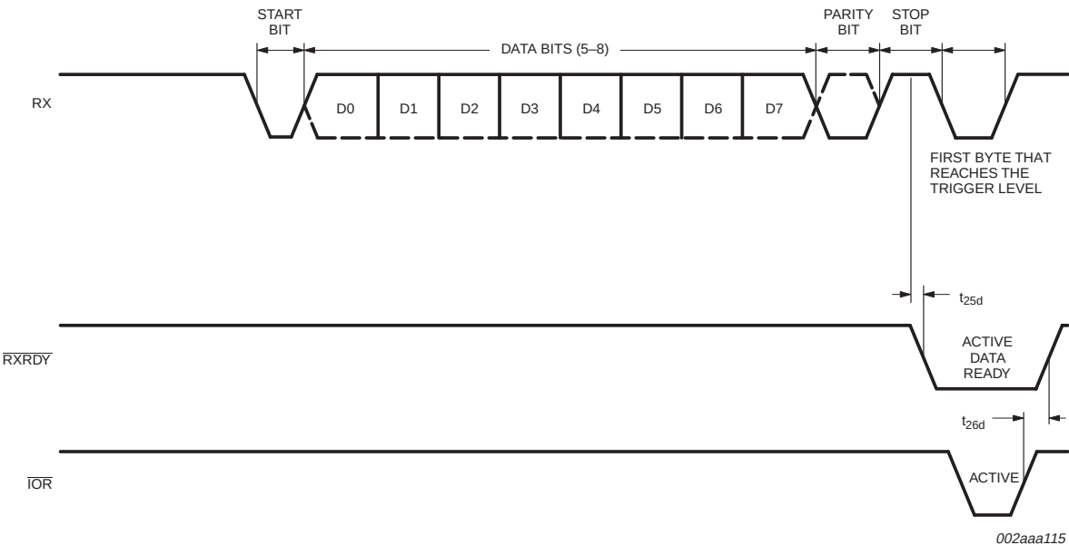
Fig 13. Receive ready timing in FIFO mode.
