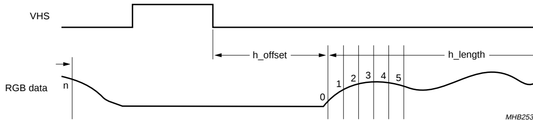
Fig.12 RGB data sampling (hsync_edge = 0).
