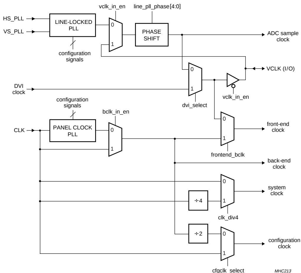
Fig.5 Clock distribution.
