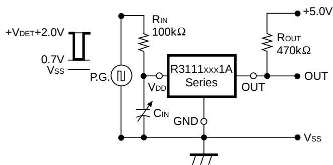
Figure 8. Output Delay Time Test Circuit (2)
