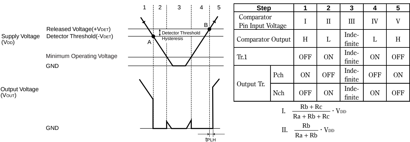
Figure 2. Operation Diagram
