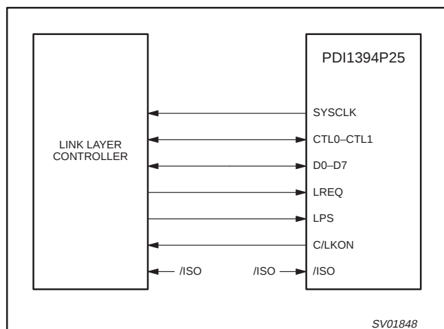
Figure 13. PHY-LLC interface
