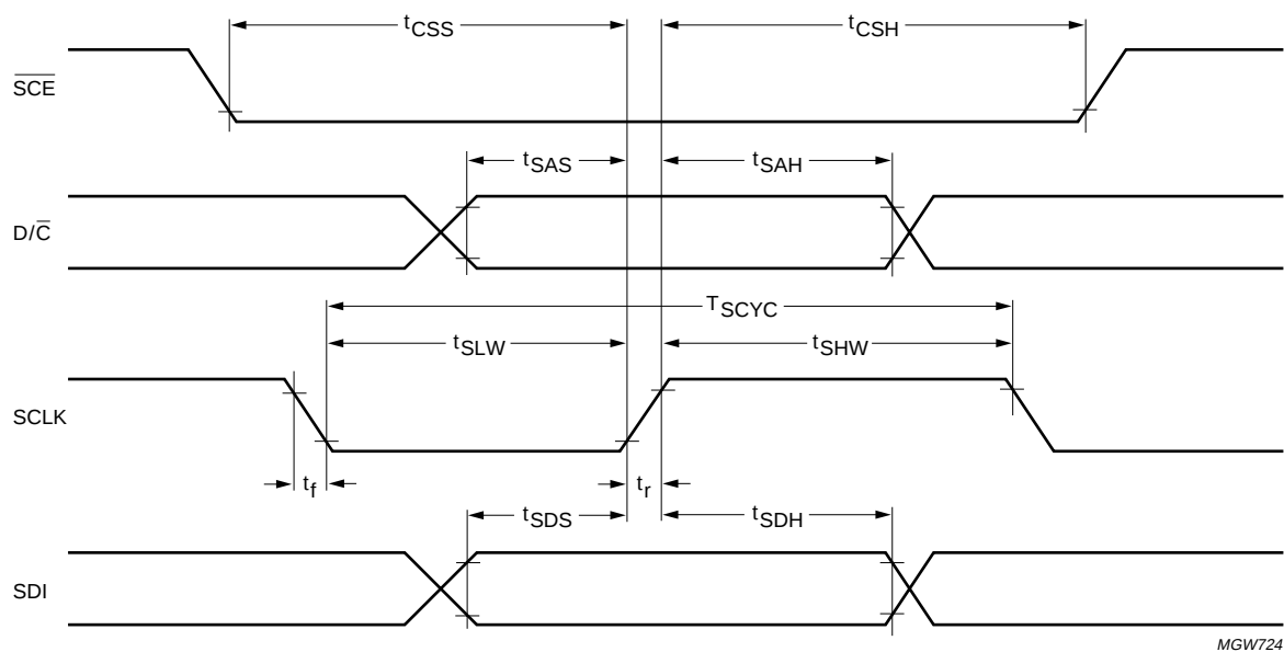
Fig.58 Serial interface timing.
