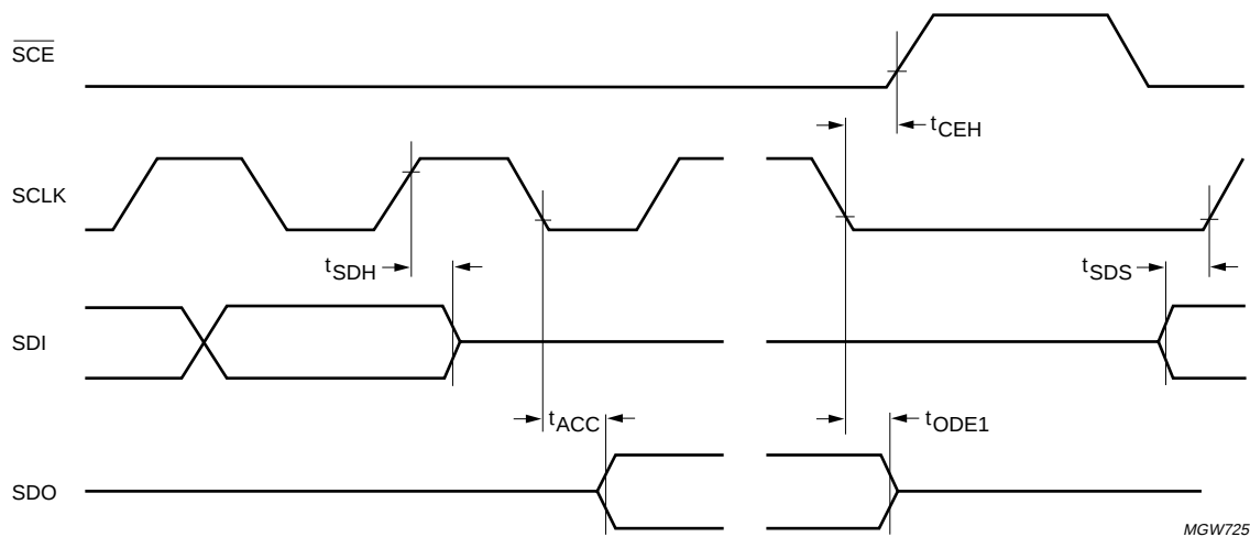
Fig.59 Serial interface timing - read mode SPI 3 or 4-line.
