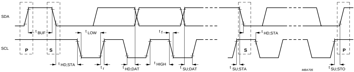
Fig 9. Timing requirements for the I 2 C-bus.
