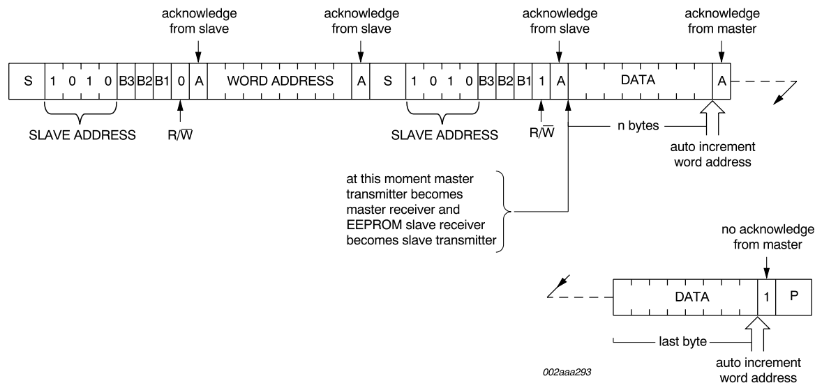
Fig 7. Master reads PCF85116-3 slave after setting word address (write word address; read data); sequential read.
