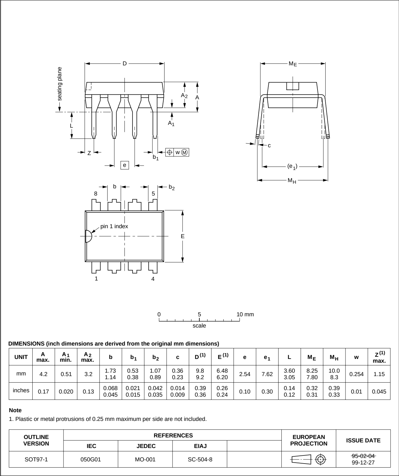
Fig 11. DIP8 (SOT97-1).
