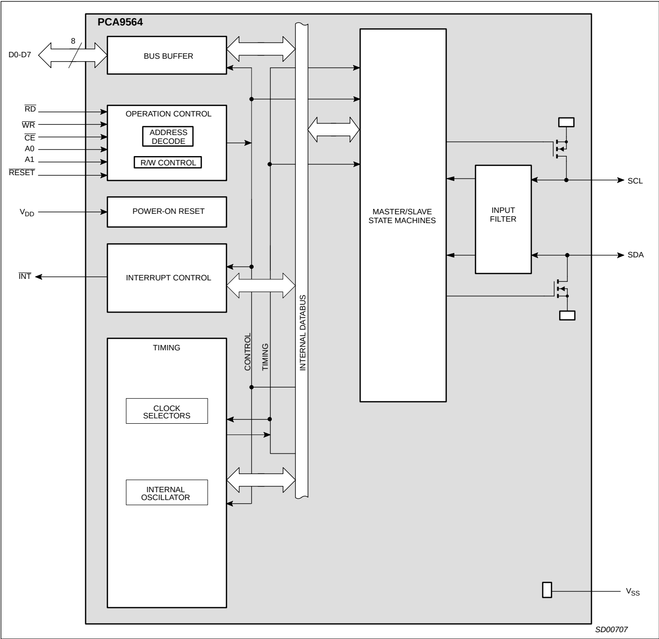
Figure 1. Block diagram
