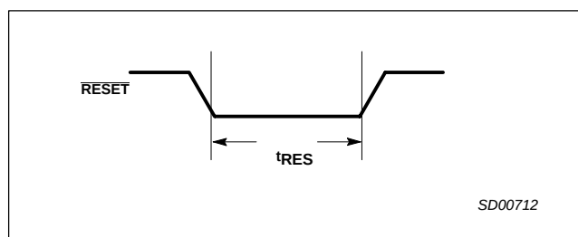
Figure 15. Reset timing
