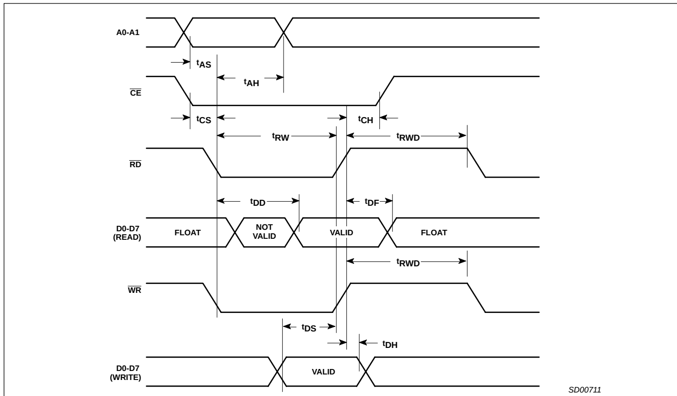
Figure 16. Bus timing
