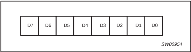
Figure 2. Control Register
