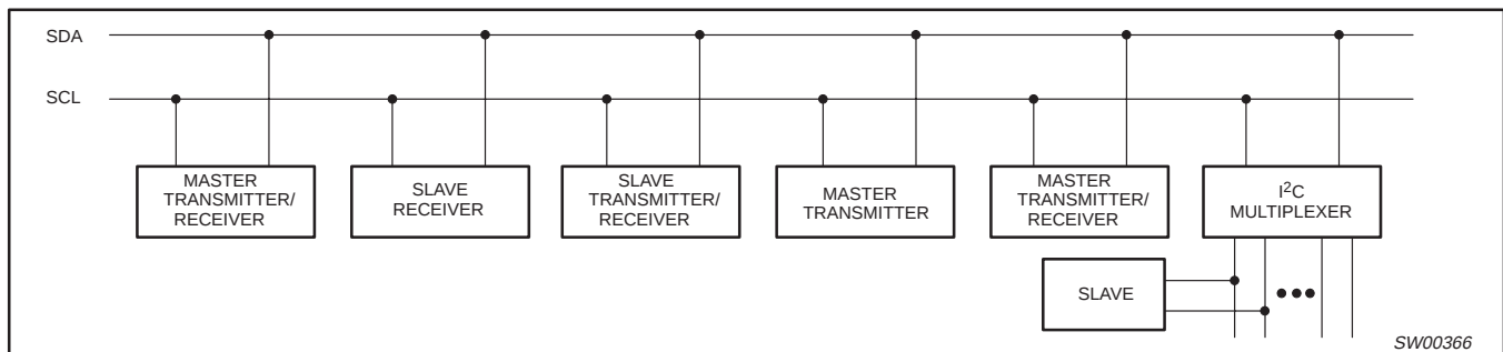
Figure 5. System configuration
