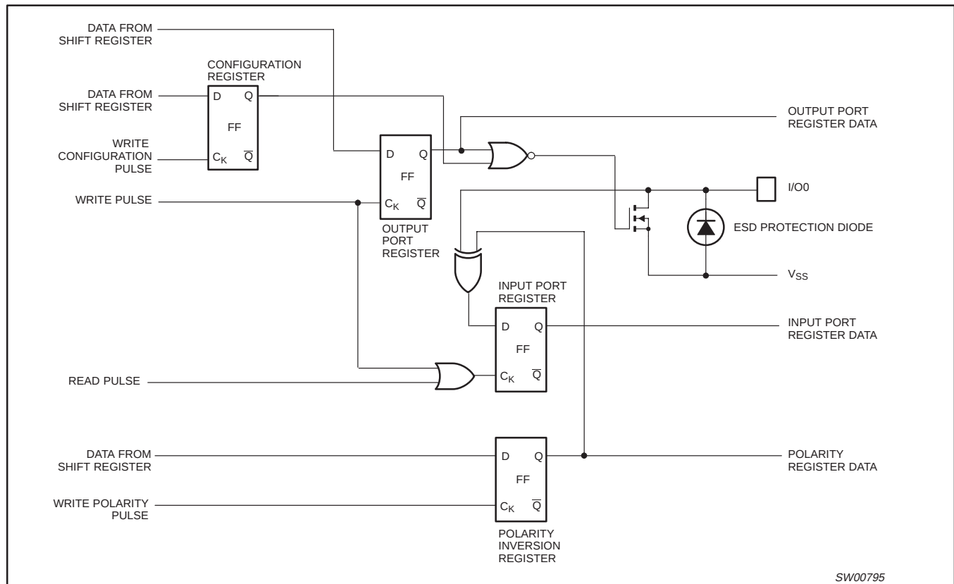
Figure 4. Simplified schematic of I/O
