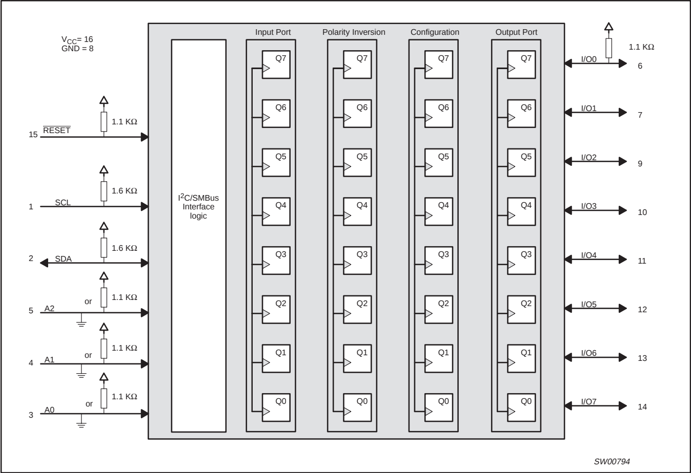
Figure 3. System diagram
