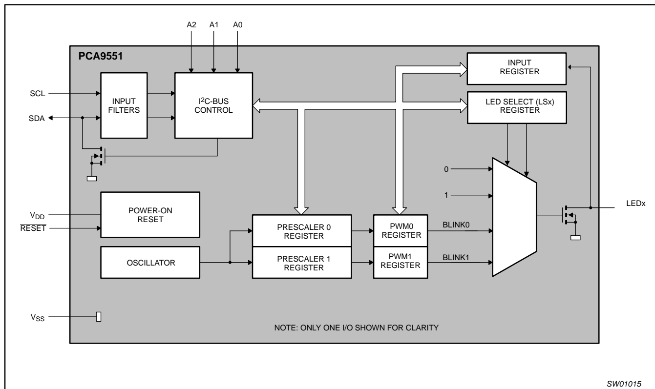
Figure 3. Block diagram
