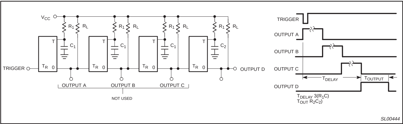
Figure 3. Long-time delay.
