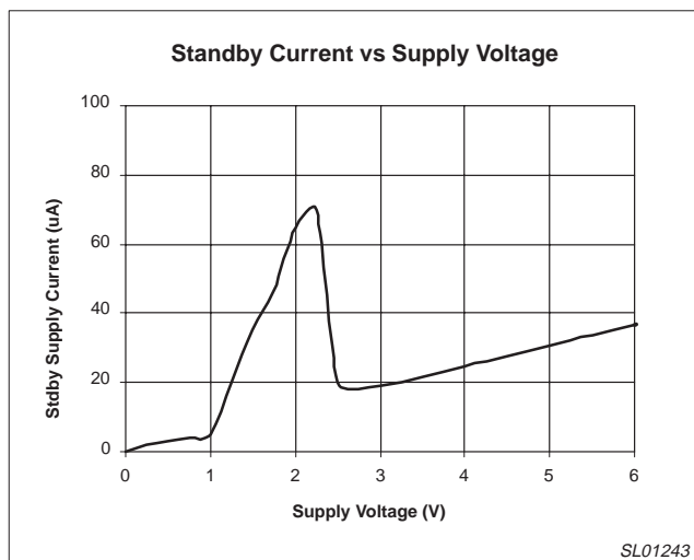
Figure 3. Standby Current versus Supply Voltage
