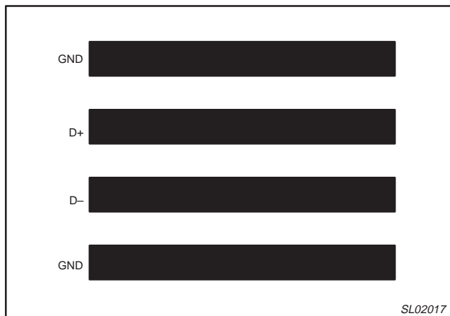
Figure 3. Ideal diode trace layout.
