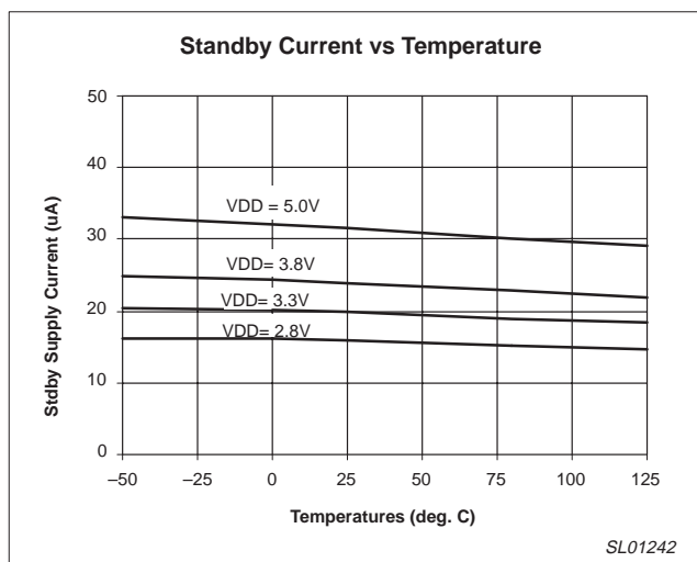
Figure 4. Standby Current versus Temperature
