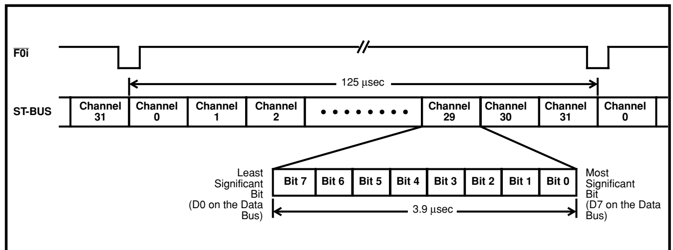
Figure 24 - ST-BUS Format
