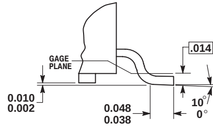
DETAIL E
