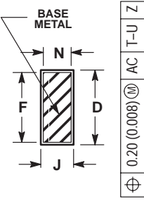
SECTION AE-AE
