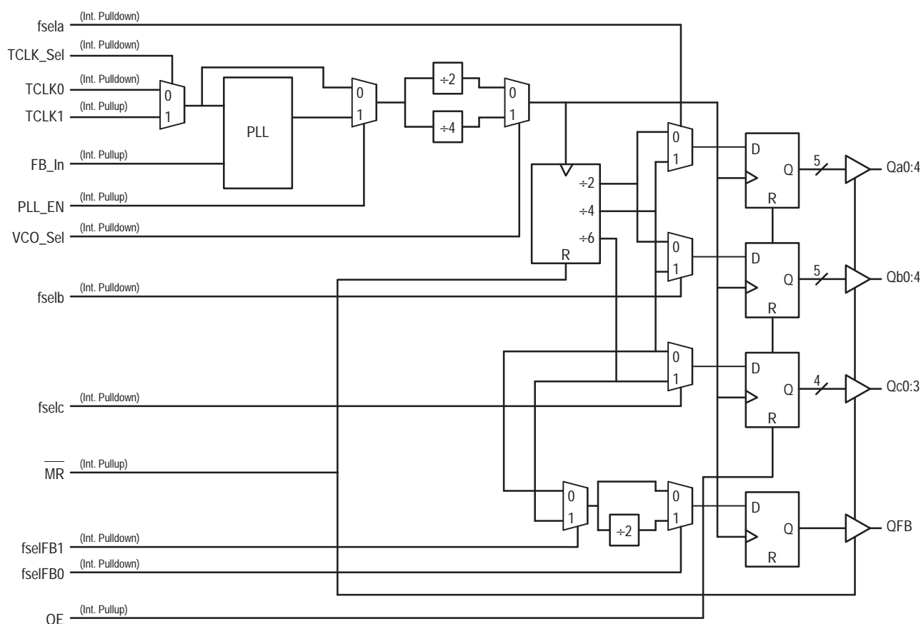
Figure 2. Logic Diagram
