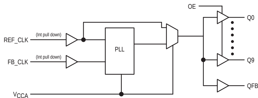
Figure 1. Block Diagram
