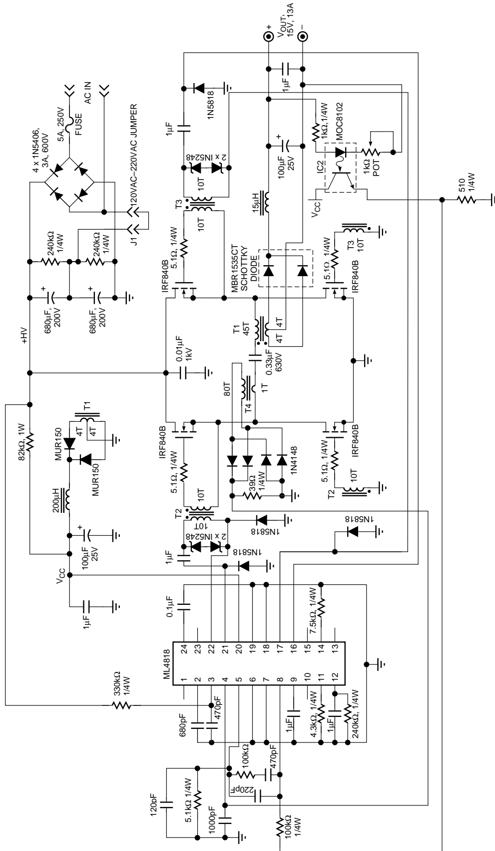
Figure 16. Offline Full Bridge Converter
