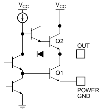
Figure 7. Power Driver Simplified Schematic
