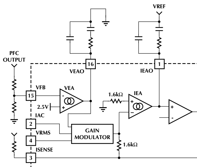
Figure 4. Compensation Network Connections for the Voltage and Current Error Amplifiers
