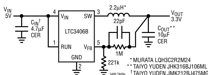
5V Input to 3.3V/0.6A Regulator
