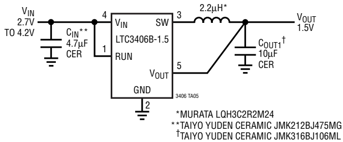
Single Li-Ion 1.5V/600mA Regulator for High Efficiency and Small Footprint
