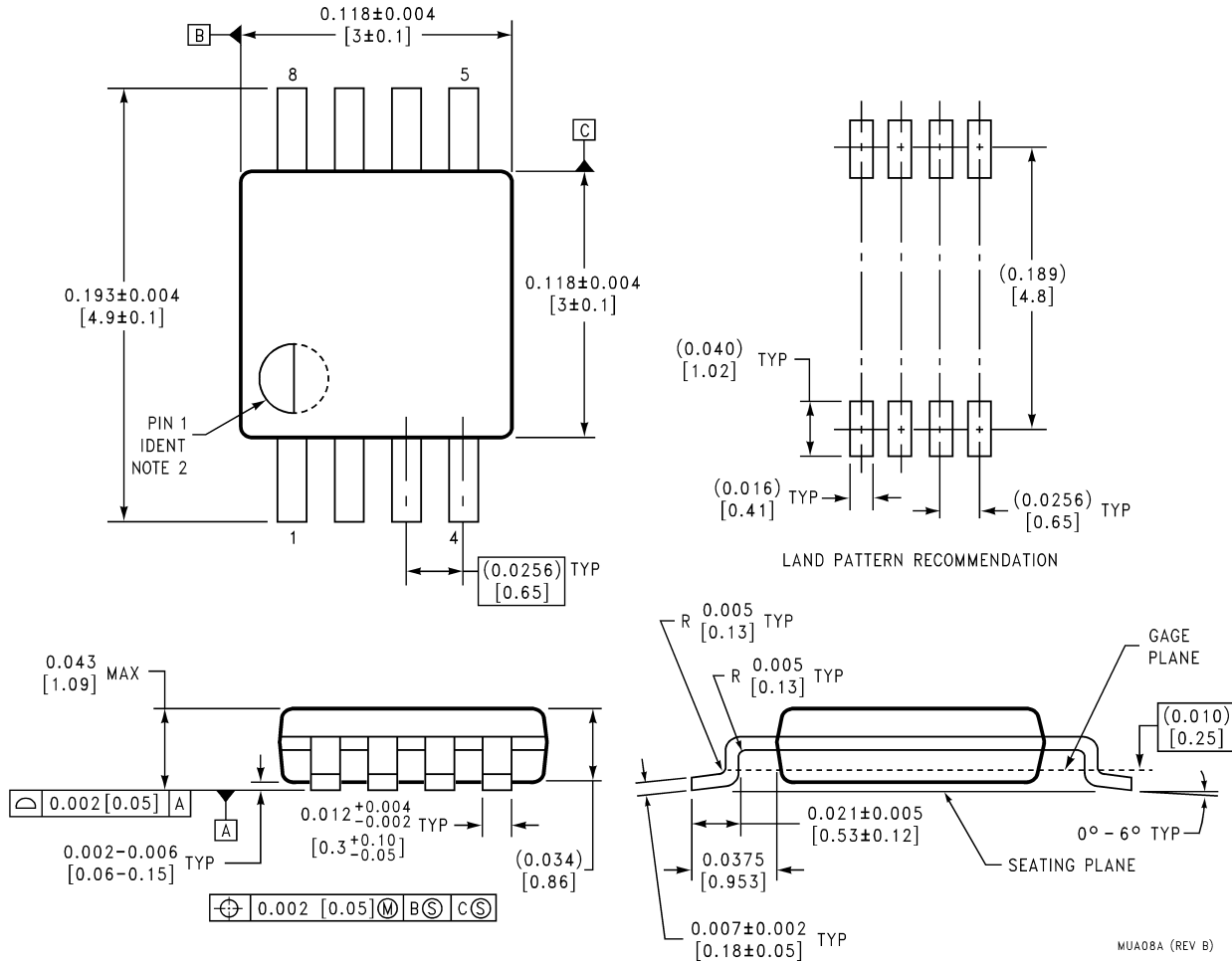
8-Lead Molded Mini Small Outline Package (MSOP) (JEDEC REGISTRATION NUMBER M0-187) Order Number LM88CIMM, or LM88CIMMX NS Package Number MUA08A
