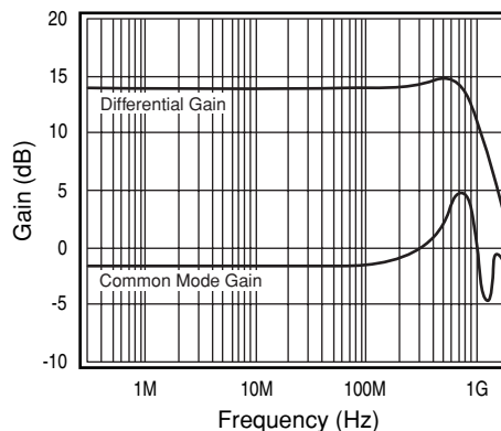
Figure 4: Differential and Common Mode Gain
