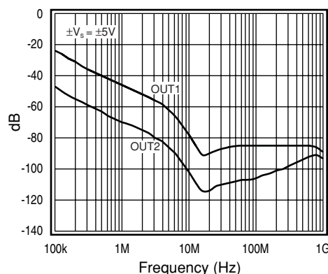
Figure 9: +V_b PSRR
