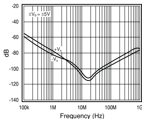
Figure 8: \pm V_s PSRR
