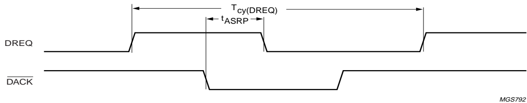
Fig 26. DMA timing in 8237 compatible mode.
