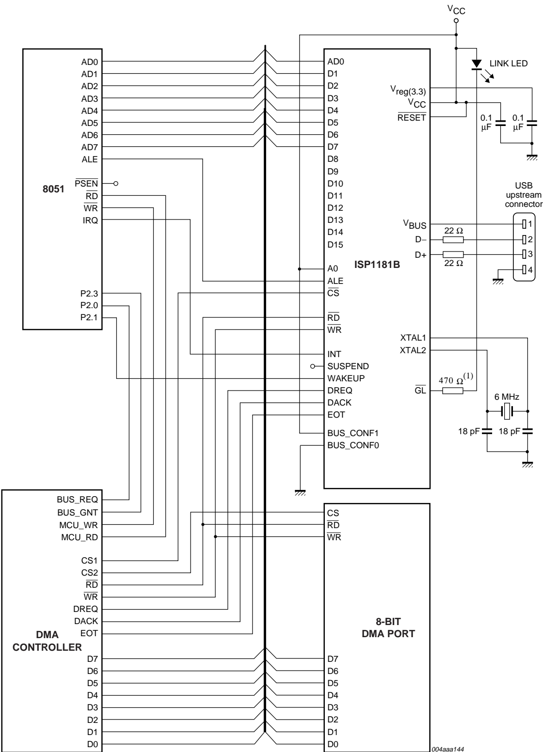
Fig 33. Typical interface circuit for bus configuration mode 2 (shared ports: 8-bit PIO, 8-bit DMA).
