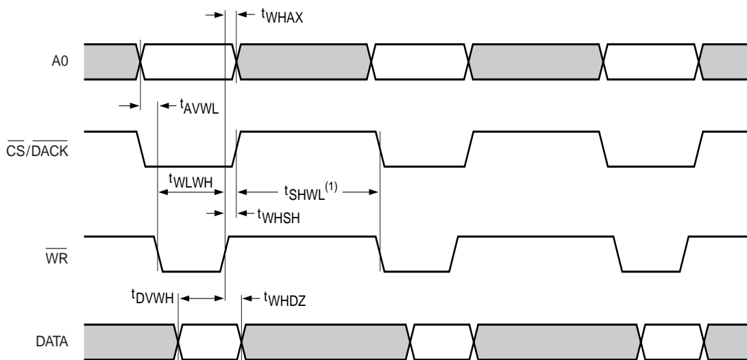
Fig 20. Parallel interface write timing (I/O and 8237 compatible DMA).
