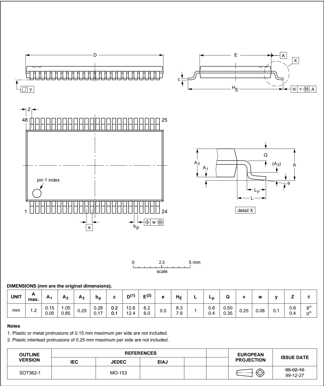
Fig 35. TSSOP48 package outline.
