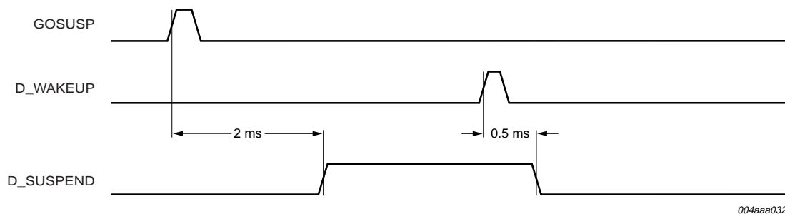
Fig 39. Suspend and resume timing for powered-off application (DC side).
