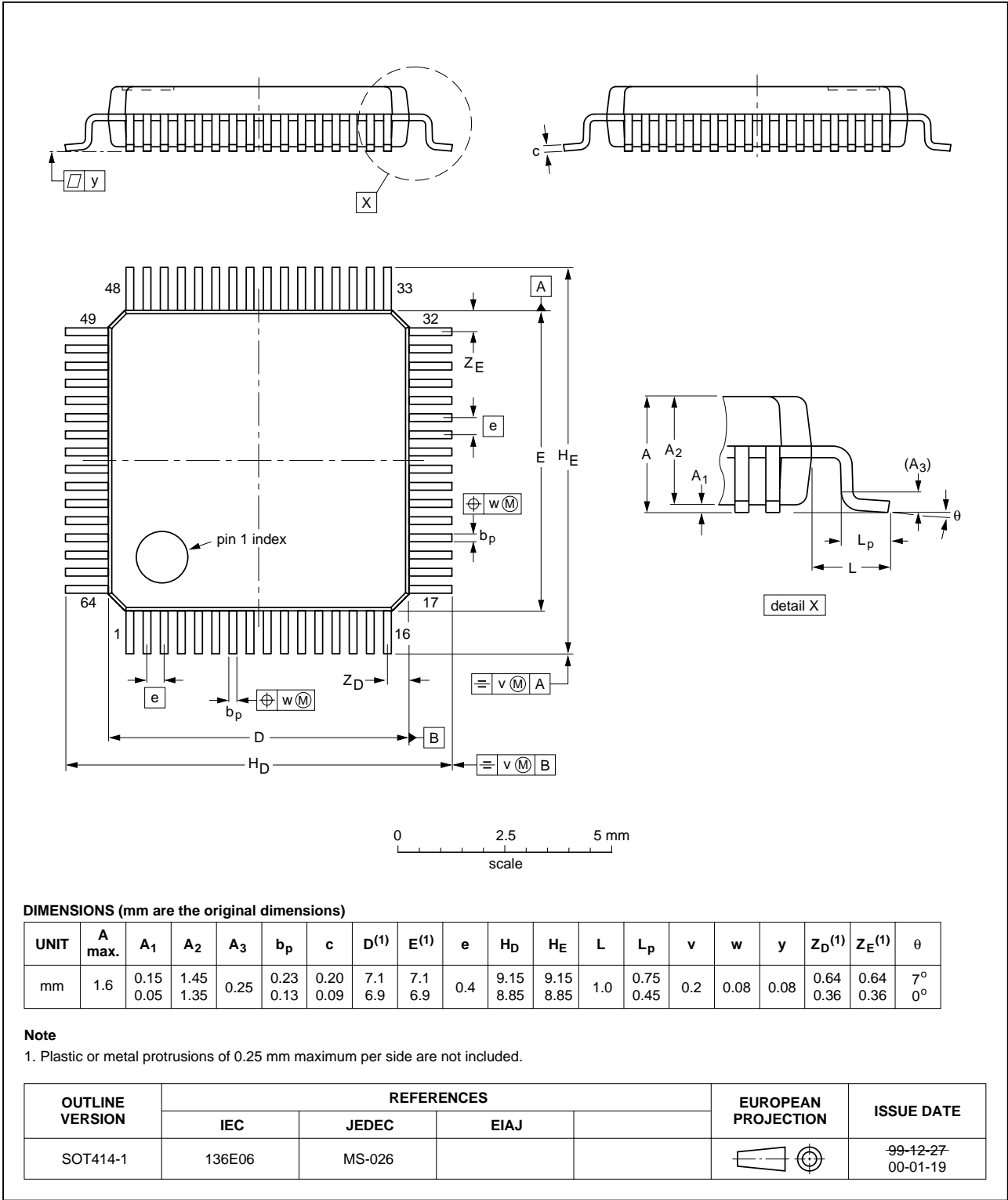
Fig 67. LQFP64 (SOT414-1) package outline.
