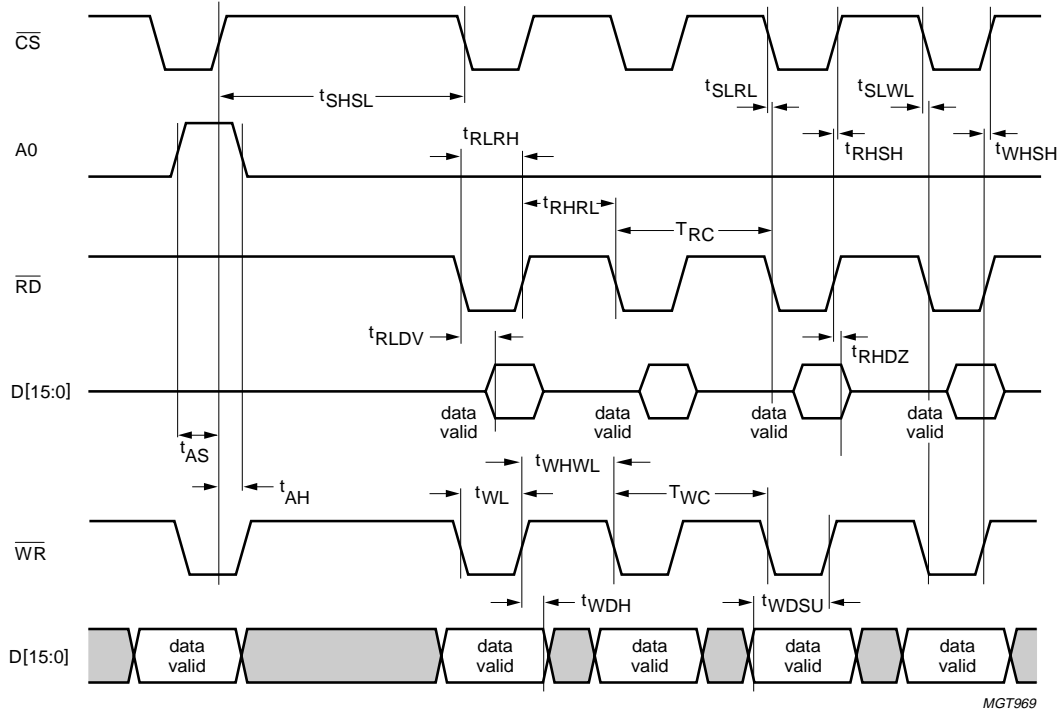
Fig 50. HC Programmed interface timing
