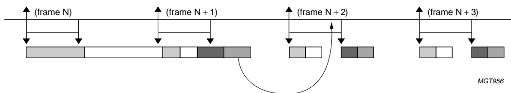
Fig 32. HC time domain behavior: example 3.
