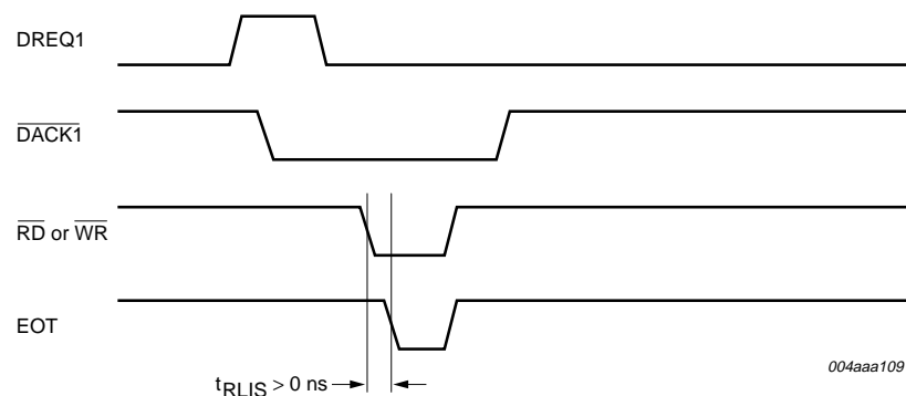
Fig 55. External EOT timing for HC single-cycle DMA.
