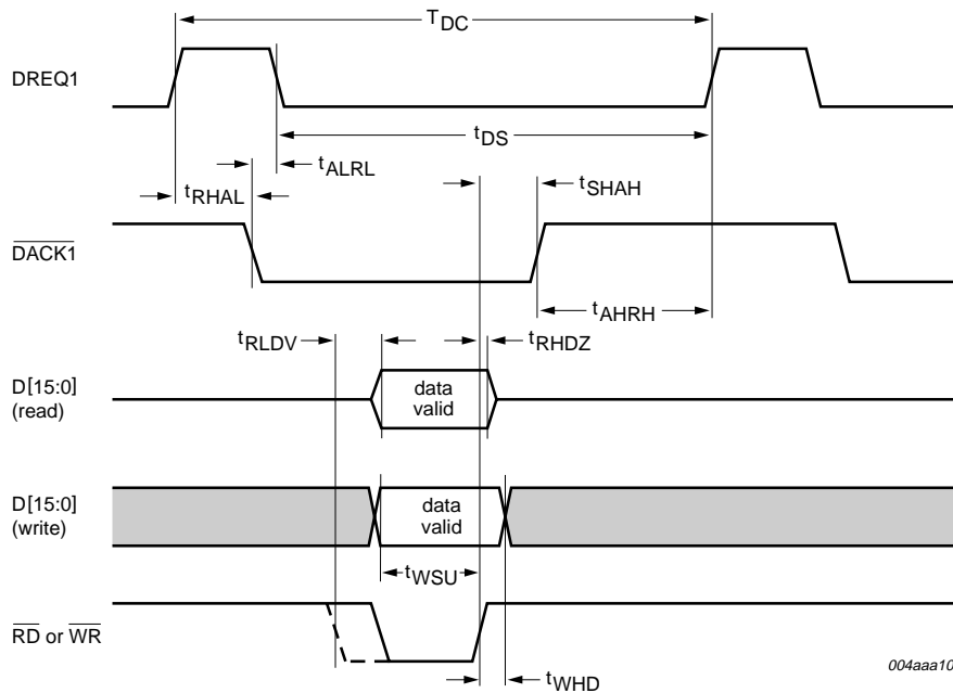
Fig 53. HC single-cycle DMA timing.
