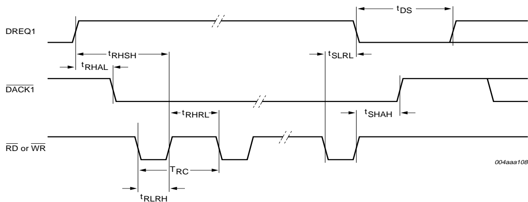
Fig 54. HC burst mode DMA timing.
