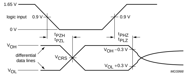
Fig 7. Timing of OE to D+, D-.
