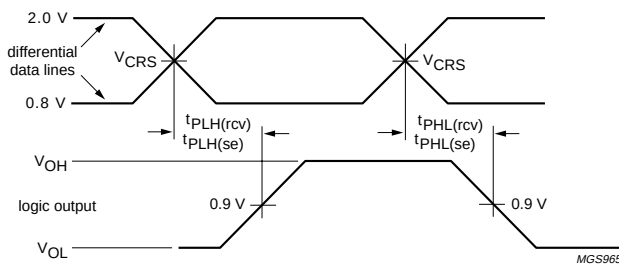
Fig 8. Timing of D+, D- to RCV, VP, VM.
