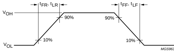
Fig 6. Rise and fall times.
