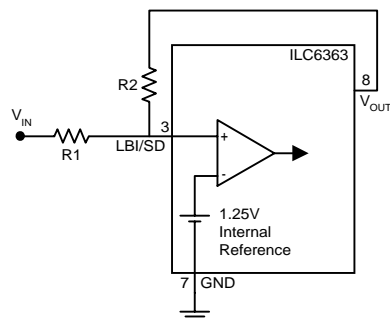
Figure 7: V_{LBI} < 1.25V
