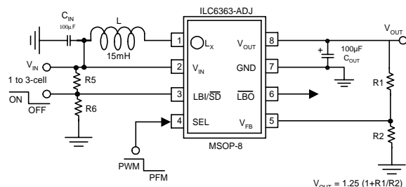
Figure 9: Adjustable Voltage Configuration
