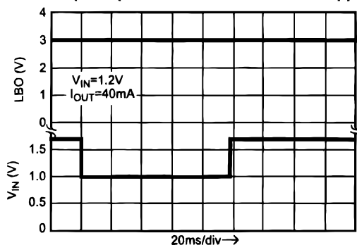
Low Battery Output ( V_{IN} < V_{TH} for Less than 100ms) 10k \Omega pull-up resistor from LBO to 3V supply
