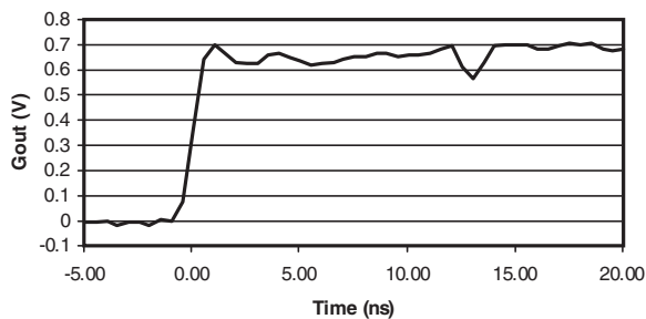
Figure 5. Matched tr.
