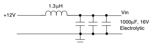
Figure 5. Input Filter
