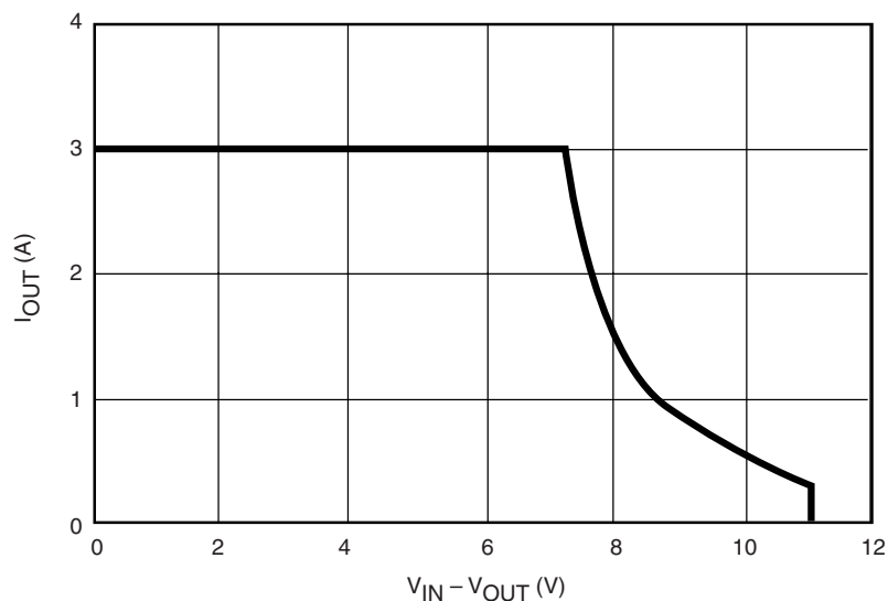
Figure 1. Absolute Maximum Safe Operating Area
