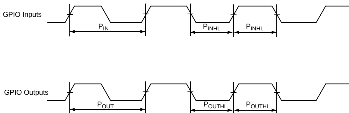
Figure 37. GPIO Timing
