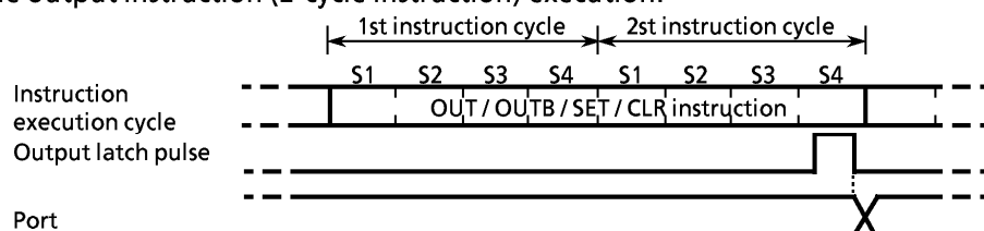
Figure 3-2. Output Timing
