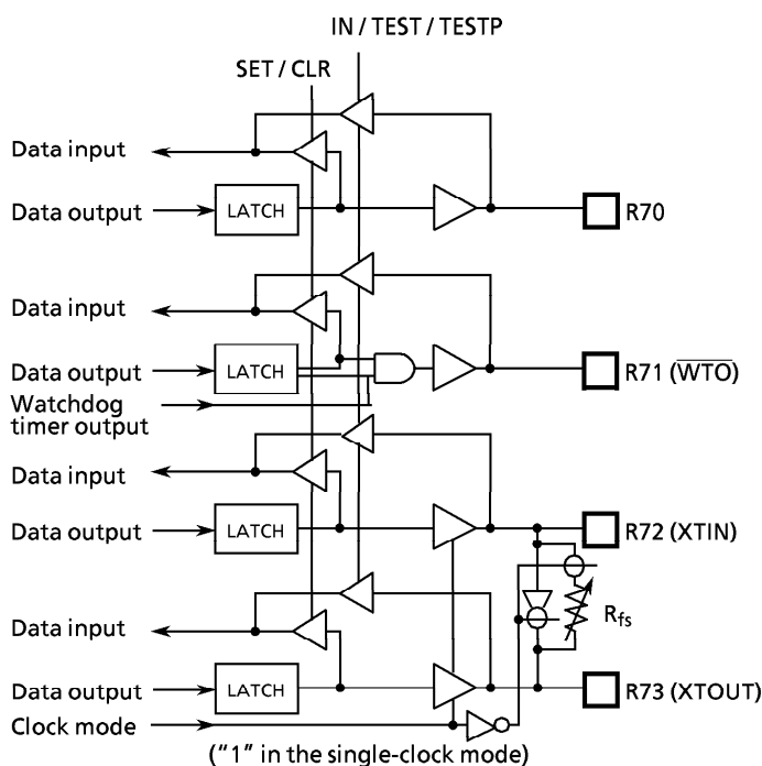
Figure 3-9. Port R7
