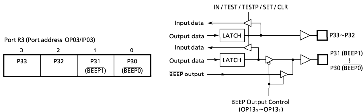
Figure 3-6. Port P3
